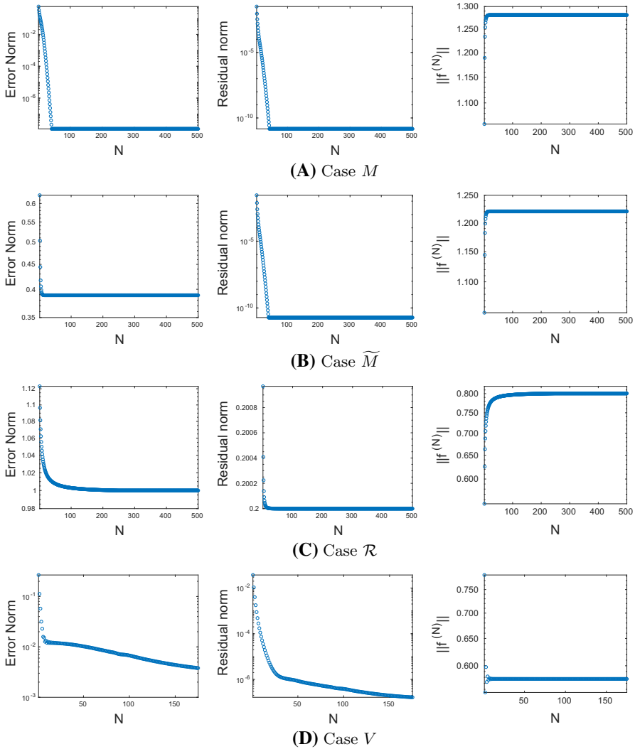
Fig. 1 Error norm and residual norm as a function of iterations for the cases of the injective multiplication operator M (baseline case), the weighted right shift \mathcal{R} , the non-injective multiplication operator \tilde{M} , and the Volterra operator V
