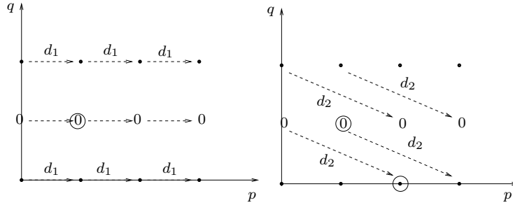
FIGURE 1. Terms E_1^{pq}(\mathcal{X}) and E_2^{pq}(\mathcal{X})
