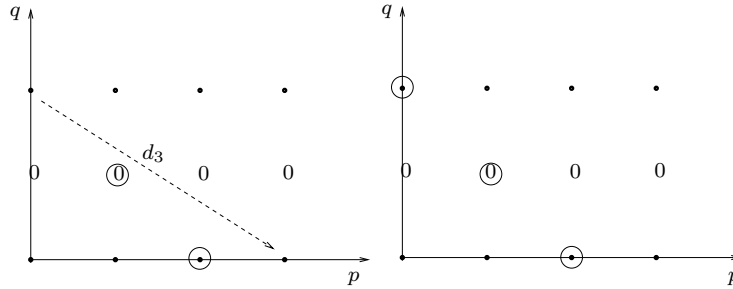
FIGURE 2. Terms E_3^{pq}(\mathcal{X}) and E_4^{pq}(\mathcal{X})
