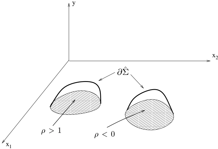
Figure 2: Two regions of y = 0 plane, one with \rho > 1 and the other with \rho < 0 , leading to a non trivial \partial\hat{\Sigma} attached to the y = 0 plane
