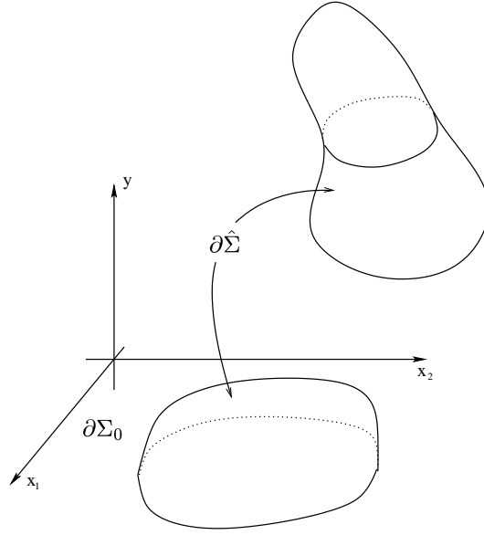
Figure 1: The domain of definition \Sigma
