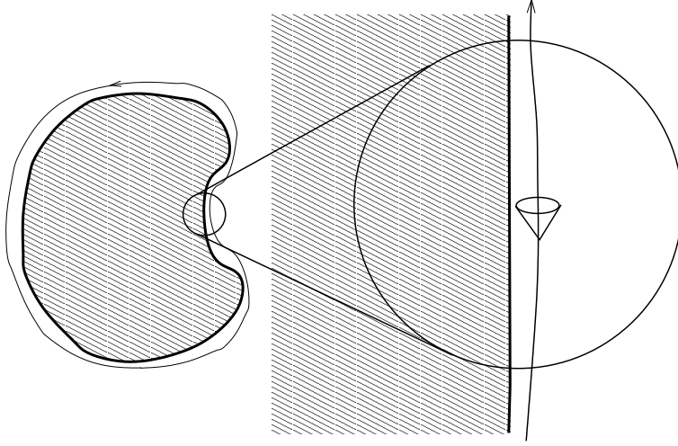
Figure 3: Zoom showing light cone near a droplet with \beta_i > 1 on the \{x_1, x_2\} plane at y = 0 .
