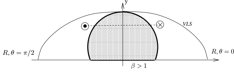
Figure 4: Singularity and velocity of light surface for a disk with \beta > 1 .
