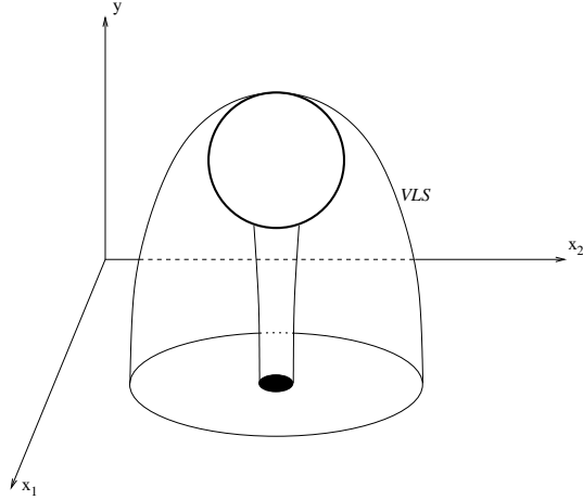
Figure 5: “Medusa” diagram: singularity, velocity of light surface and cylinder connecting the singularity ( \partial\hat{\Sigma} ) to the y = 0 plane, for the lifted sphere.
