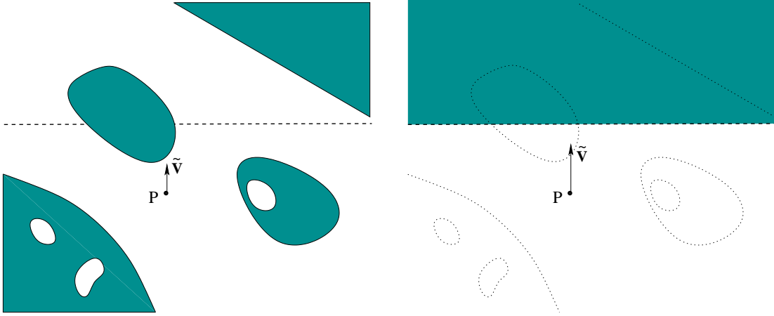
Figure 7: Changing \mathcal{D} into \Pi
