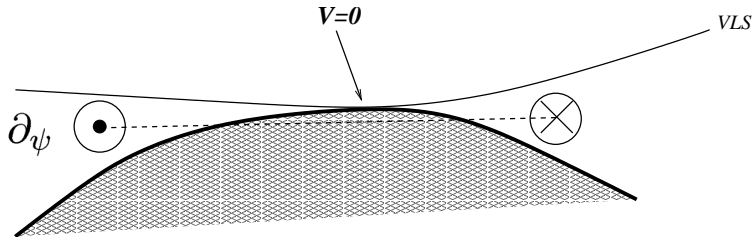
Figure 6: \partial\hat{\Sigma} and the VLS touching at V^2 = 0 .
