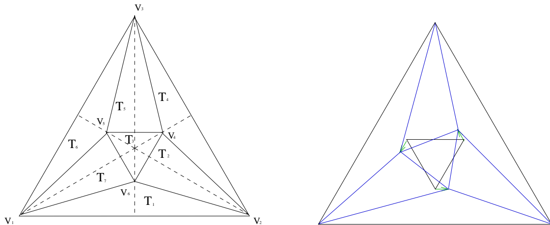
FIGURE 4.1. Triangle T and a prototype of a piecewise affine vector field u such that \operatorname{div} u = 0 a.e. in T and u = 0 on \partial T .
