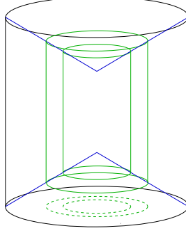
FIGURE 3.1. Illustration of the sets K_0^m , \mathcal{C}_m and U_i appearing in the proof of Theorem 3.6, in the (a_1, a_2, a_3) -space. U_i is the region between the two small cylinders, coloured in green.
