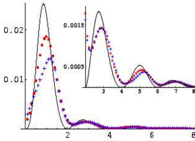
Figure 3: Process quark+anti-quark \rightarrow closed-string(missing)+gluon, cross-section in units of \alpha' , as a function of \alpha's .
