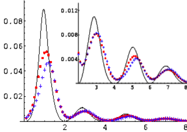
Figure 2: Process gluon+gluon \rightarrow closed-string(missing)+gluon, cross-section in units of \alpha' , as a function of \alpha's .
